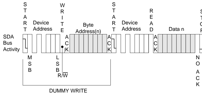
Figure 5-9. Random Address Read
