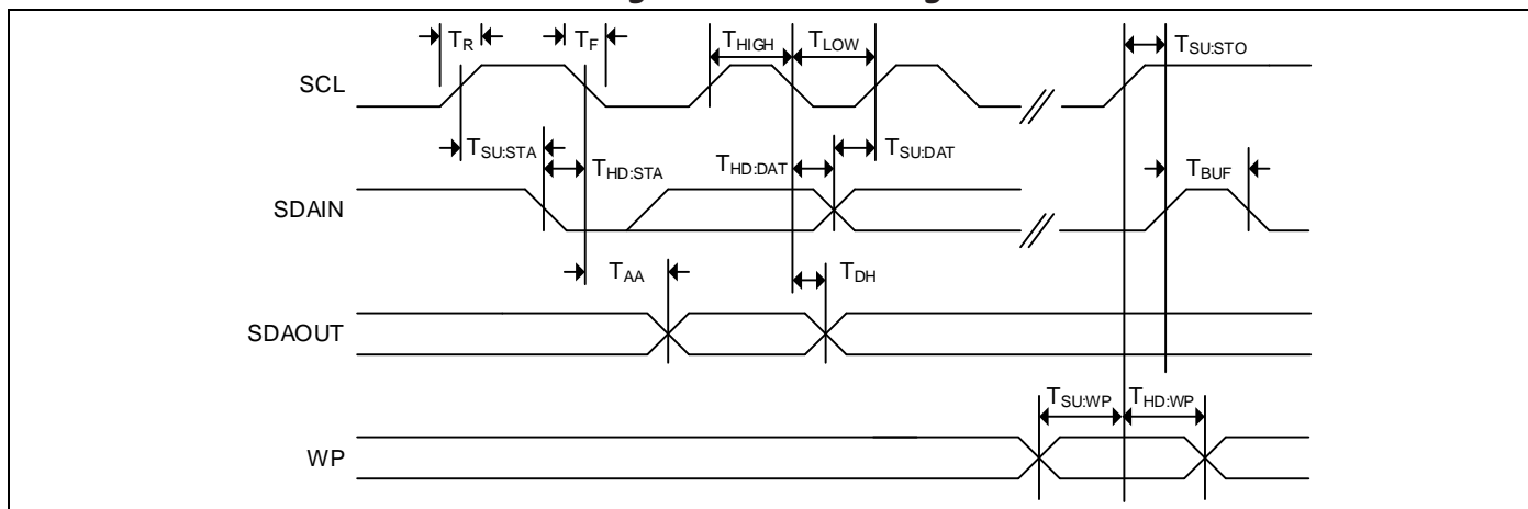
Figure 5-11. Bus Timing
