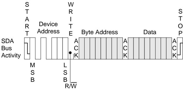
Figure 5-6. Byte Write
