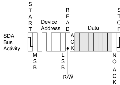
Figure 5-8. Current Address Read
