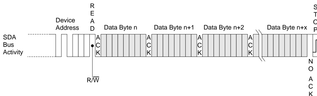
Figure 5-10. Sequential Read
